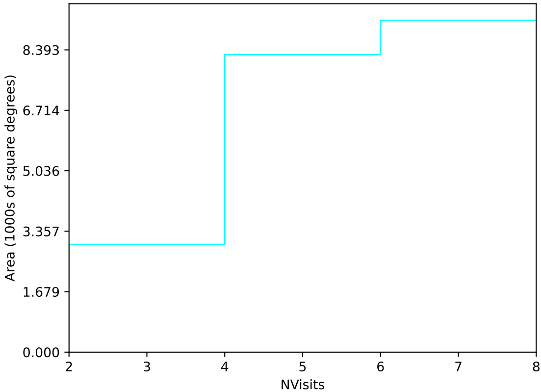
weather_cloudso36v3.4_10yrs Yr 1 u band: NVisits
