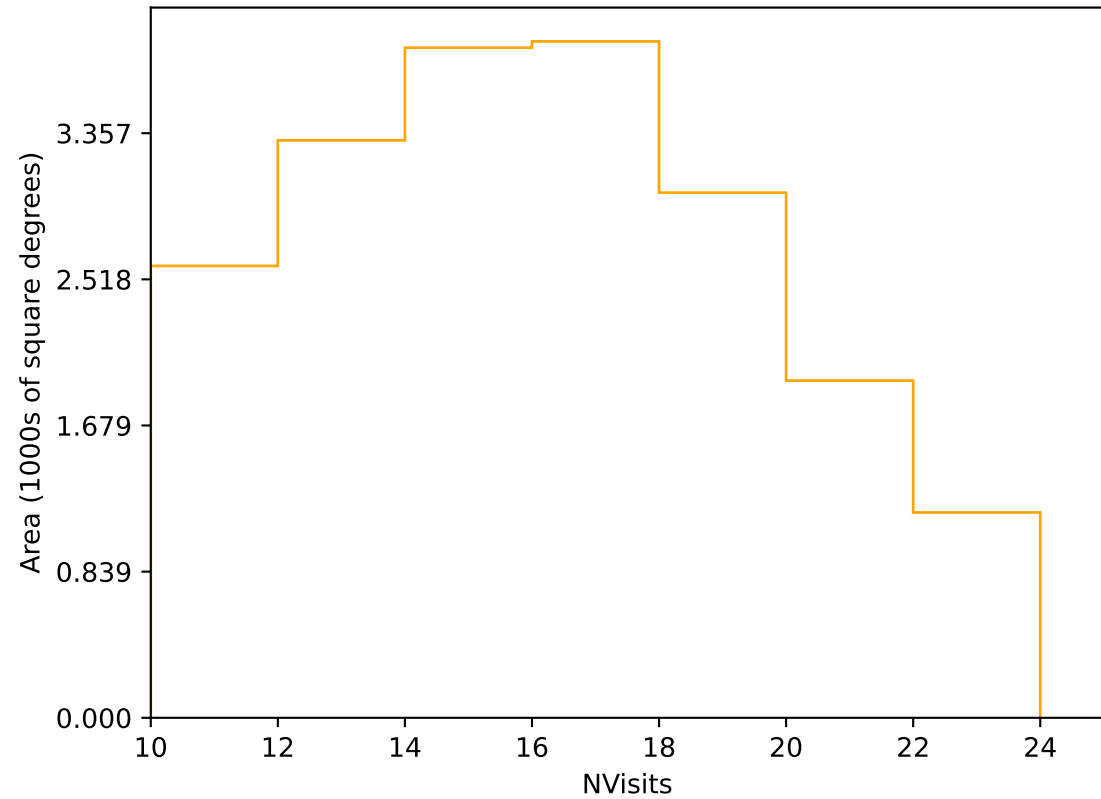
weather_cloudso36v3.4_10yrs Yr 1 r band: NVisits
