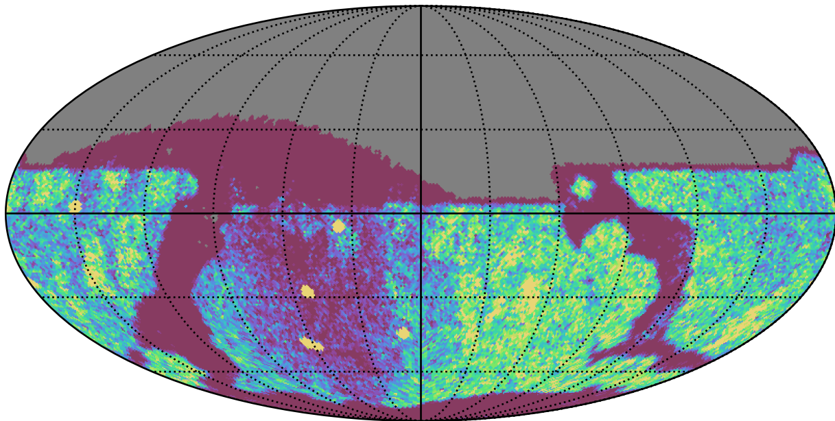
weather_cloudso36v3.4_10yrs Yr 1 i band: NVisits
