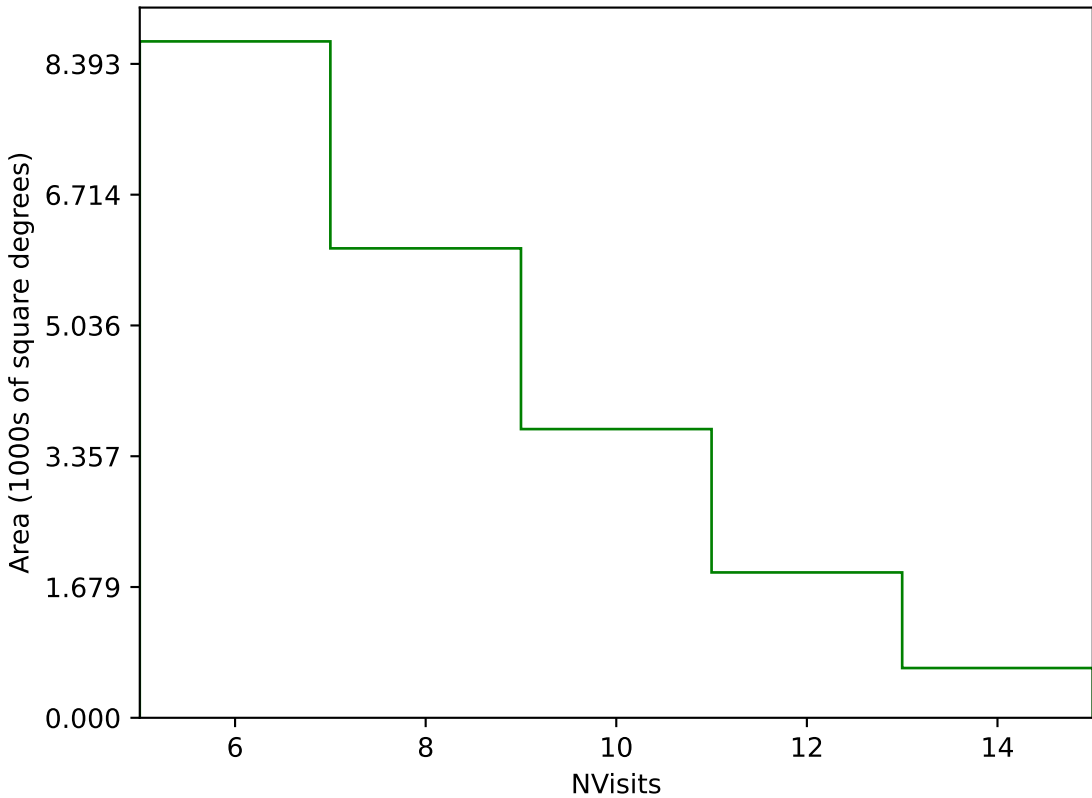
weather_cloudso36v3.4_10yrs Yr 1 g band: NVisits
