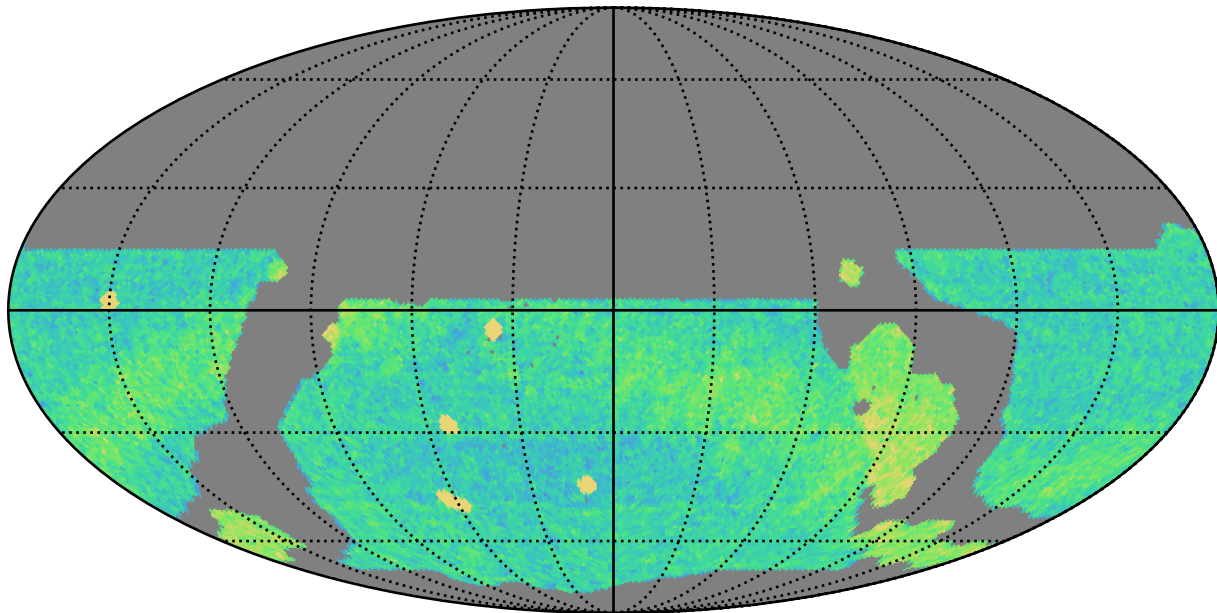
weather_cloudso36v3.4_10yrs WFD r band: NVisits
