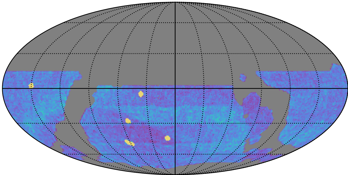
weather_cloudso36v3.4_10yrs WFD all bands: NVisits
