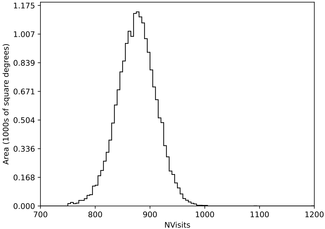
weather_cloudso36v3.4_10yrs WFD all bands: NVisits
