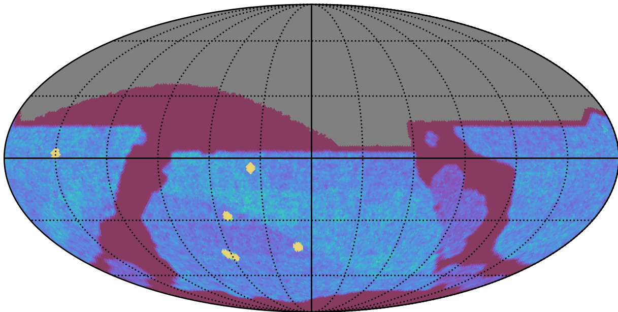
weather_cloudso36v3.4_10yrs All sky z band: NVisits
