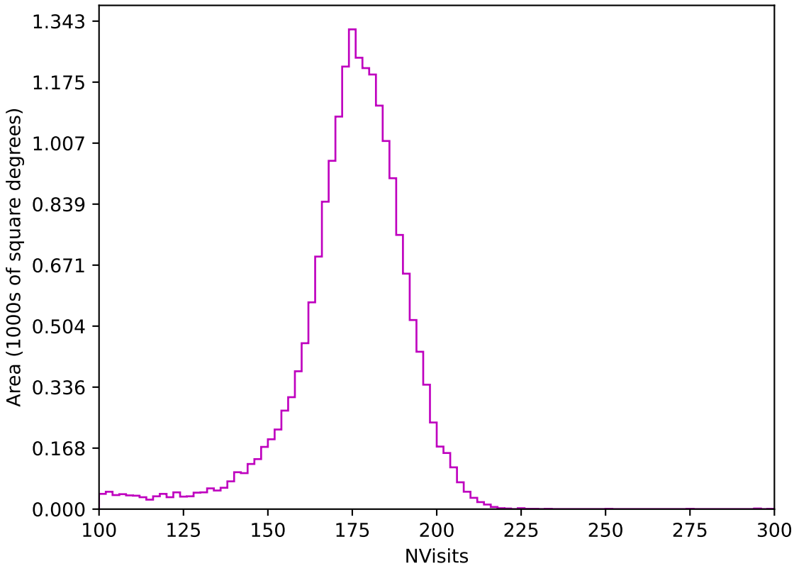
weather_cloudso36v3.4_10yrs All sky z band: NVisits
