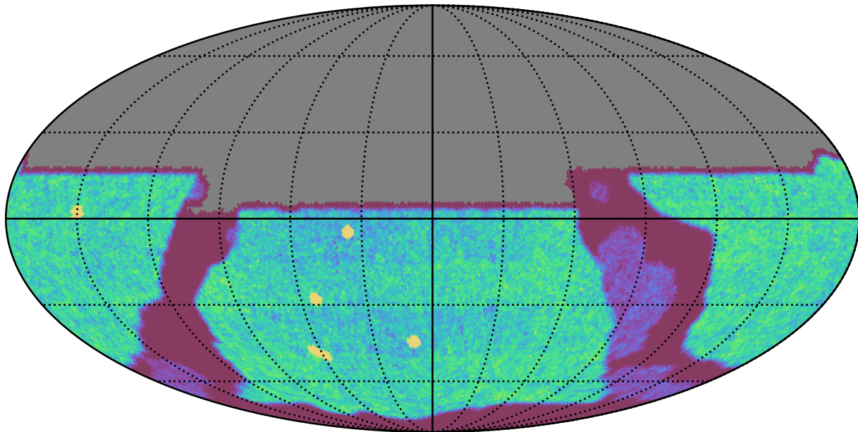
weather_cloudso36v3.4_10yrs All sky u band: NVisits
