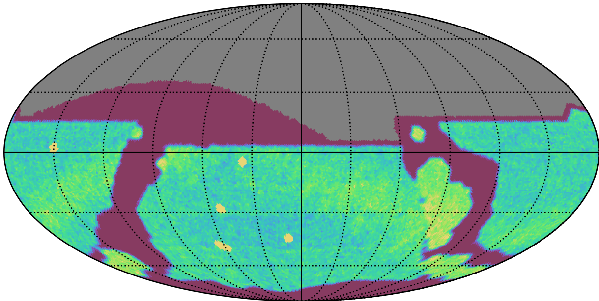
weather_cloudso36v3.4_10yrs All sky r band: NVisits
