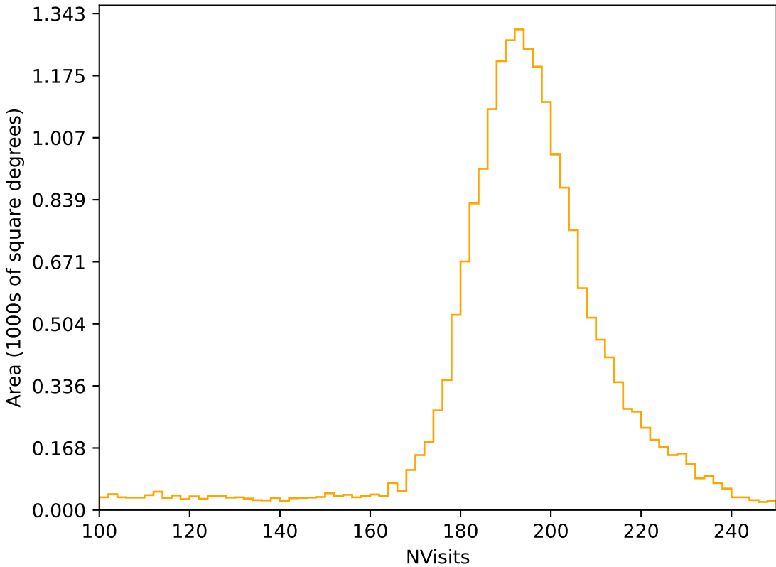
weather_cloudso36v3.4_10yrs All sky r band: NVisits
