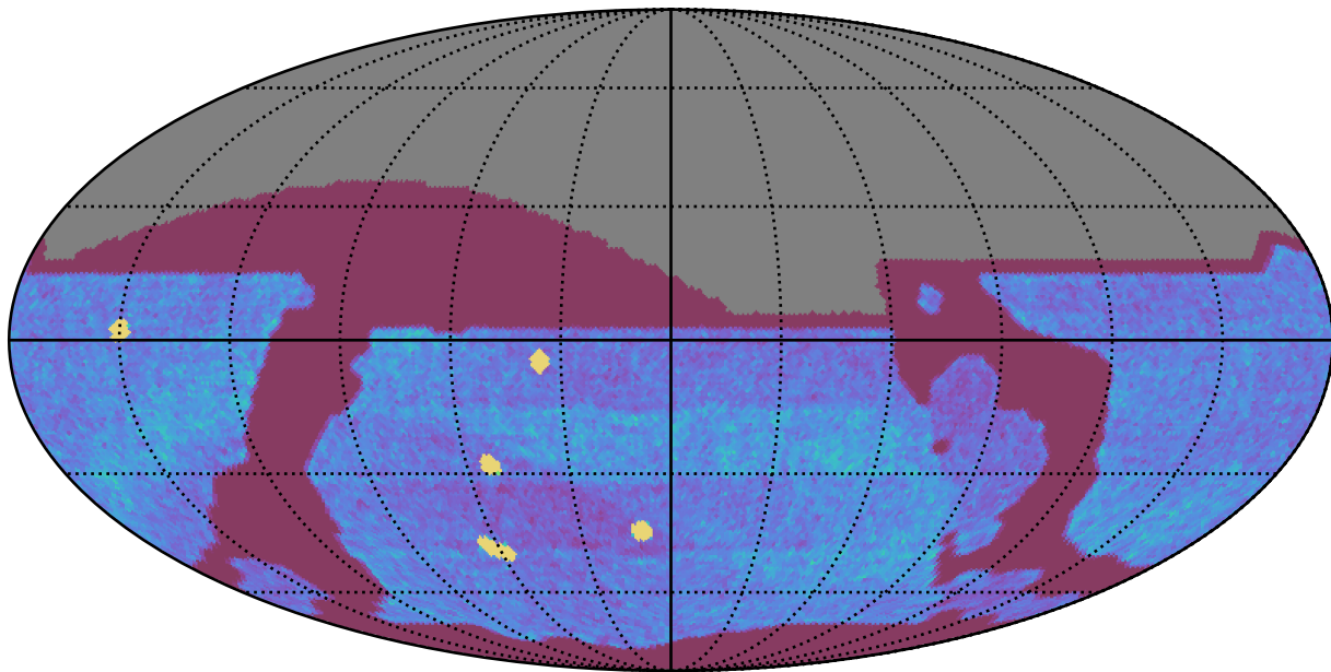
weather_cloudso36v3.4_10yrs All sky all bands: NVisits
