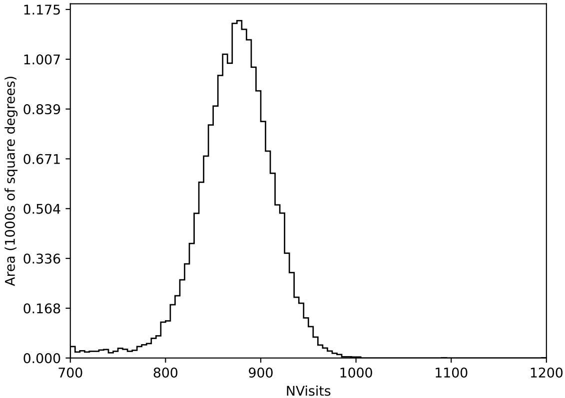
weather_cloudso36v3.4_10yrs All sky all bands: NVisits
