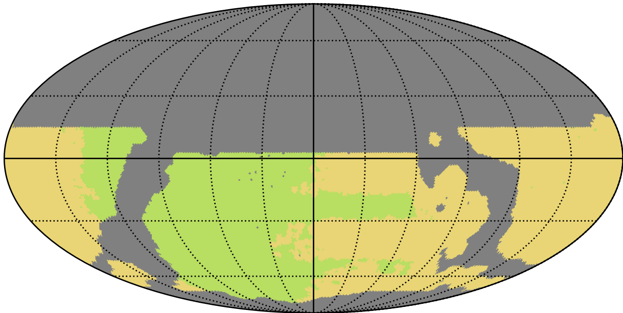
weather_cloudso36v3.4_10yrs WFD all bands: NSeasons
