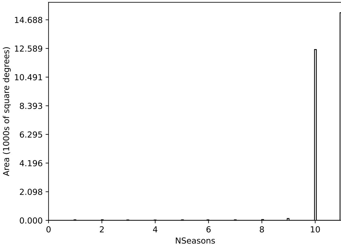
weather_cloudso36v3.4_10yrs All sky all bands: NSeasons
