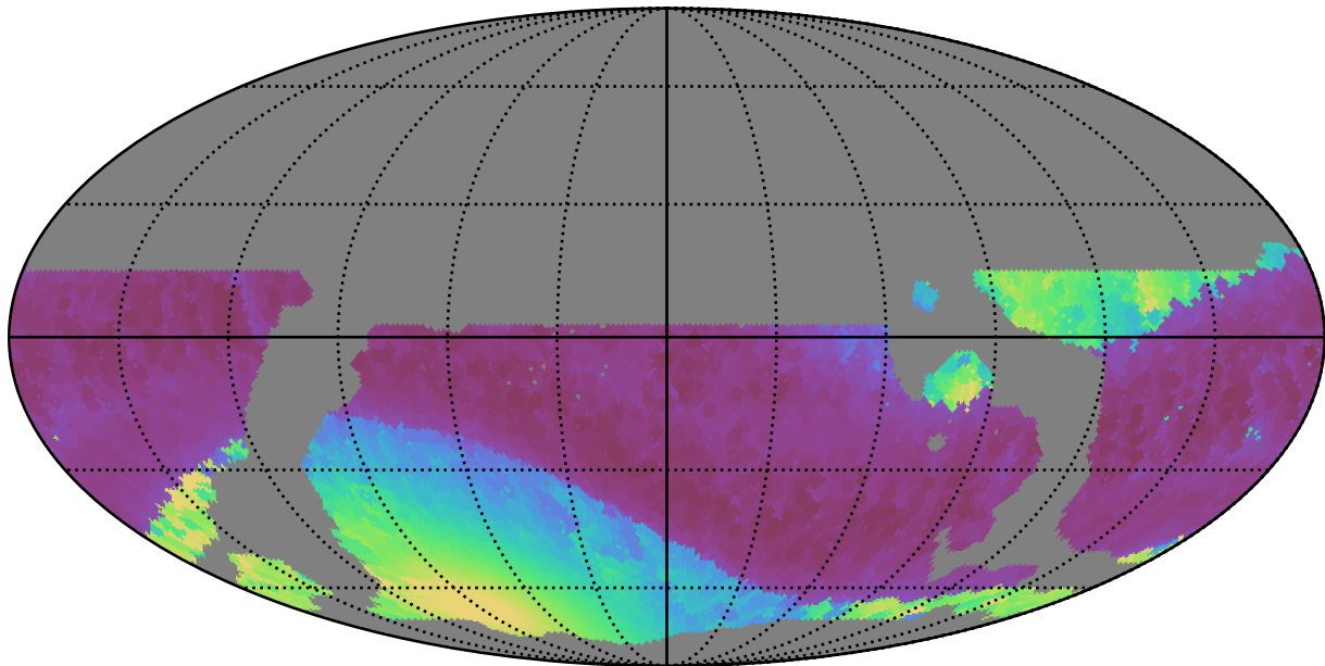
weather_cloudso36v3.4_10yrs WFD all bands: Min solarElong
