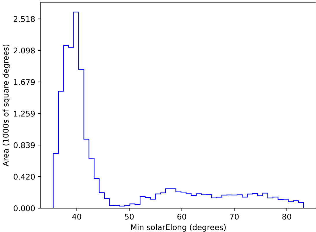
weather_cloudso36v3.4_10yrs WFD all bands: Min solarElong
