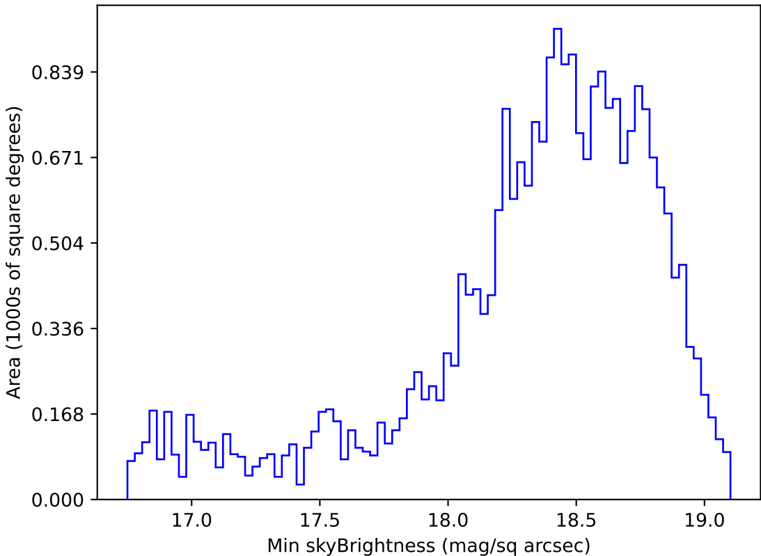
weather_cloudso36v3.4_10yrs Yr 1 z band: Min skyBrightness
