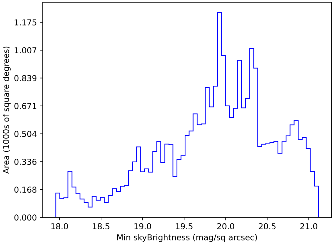
weather_cloudso36v3.4_10yrs Yr 1 r band: Min skyBrightness
