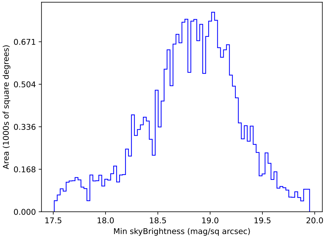
weather_cloudso36v3.4_10yrs Yr 1 i band: Min skyBrightness
