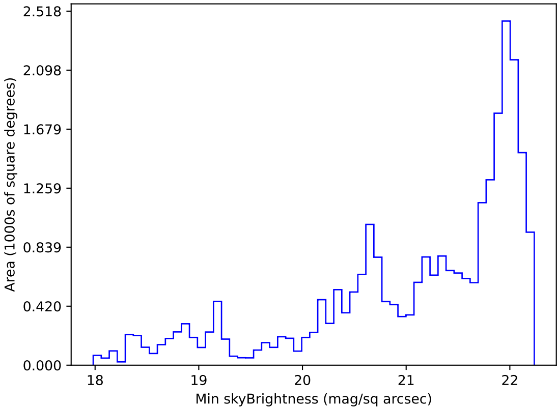
weather_cloudso36v3.4_10yrs Yr 1 g band: Min skyBrightness
