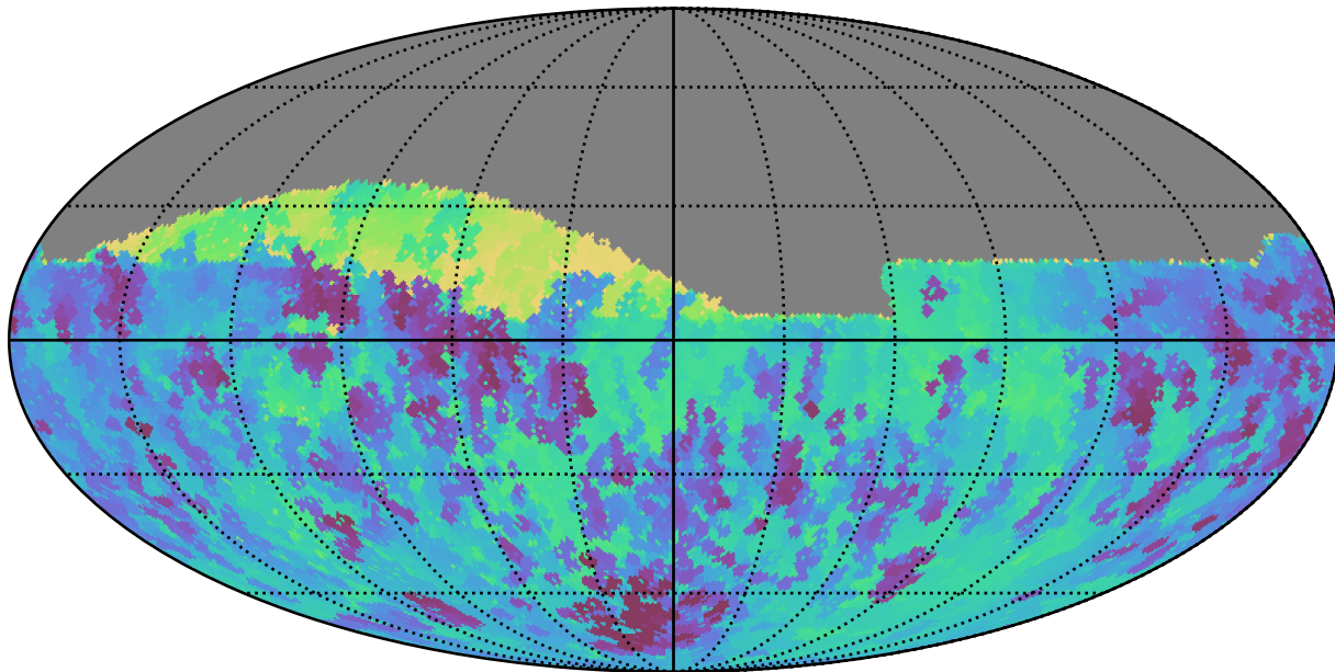
weather_cloudso36v3.4_10yrs Yr 1 all bands: Min skyBrightness
