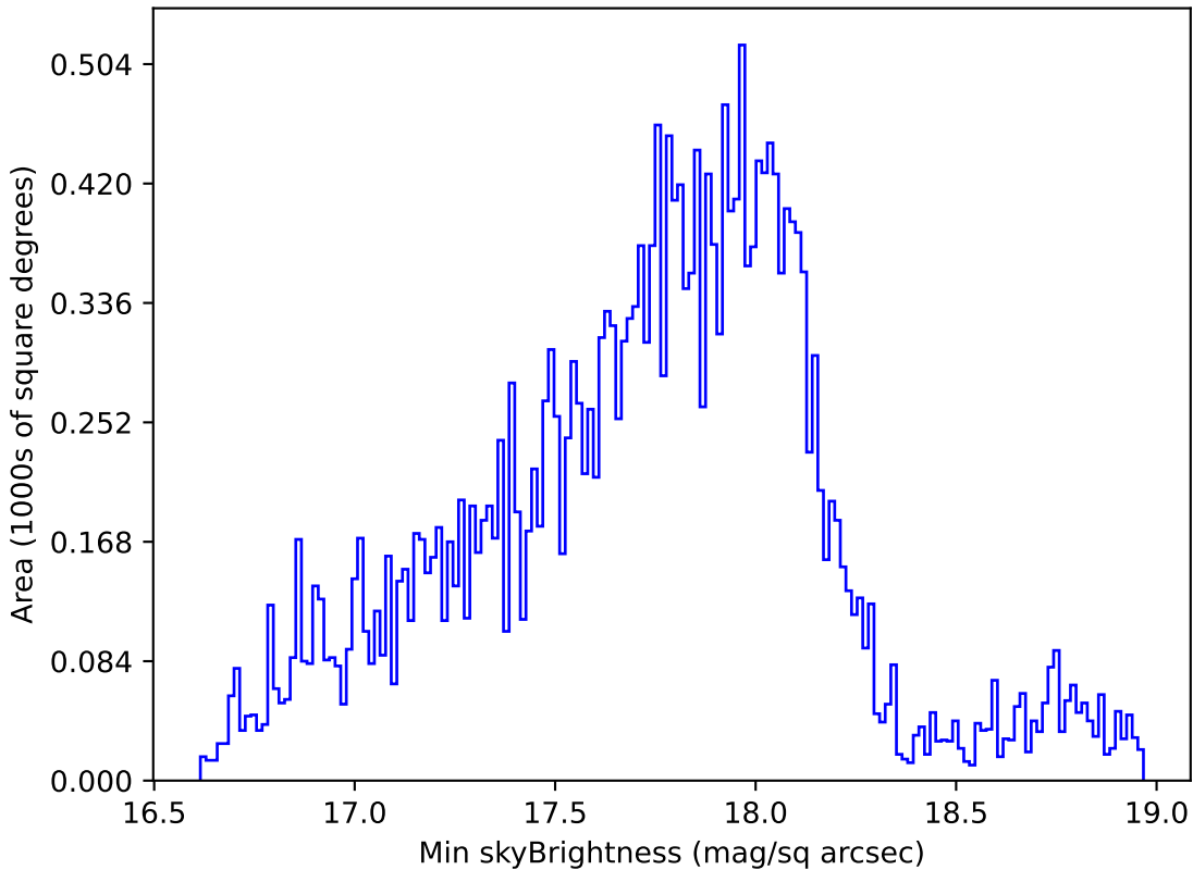
weather_cloudso36v3.4_10yrs Yr 1 all bands: Min skyBrightness
