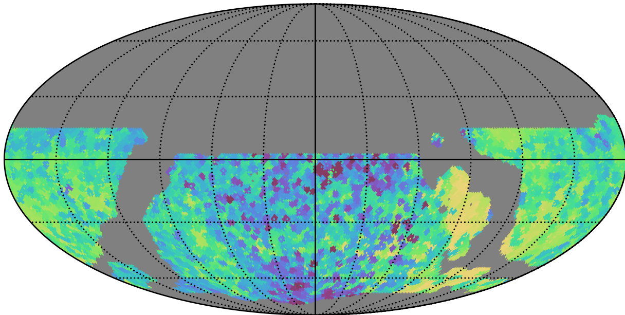
weather_cloudso36v3.4_10yrs WFD y band: Min skyBrightness
