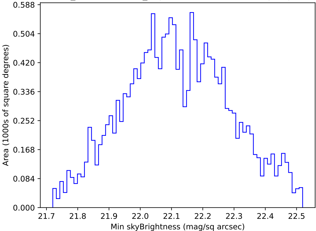
weather_cloudso36v3.4_10yrs WFD u band: Min skyBrightness
