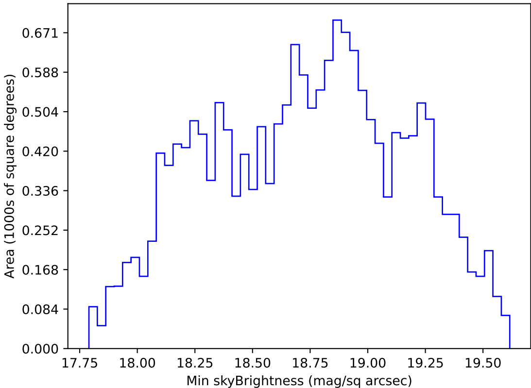
weather_cloudso36v3.4_10yrs WFD r band: Min skyBrightness
