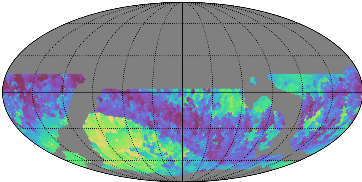
weather_cloudso36v3.4_10yrs WFD i band: Min skyBrightness
