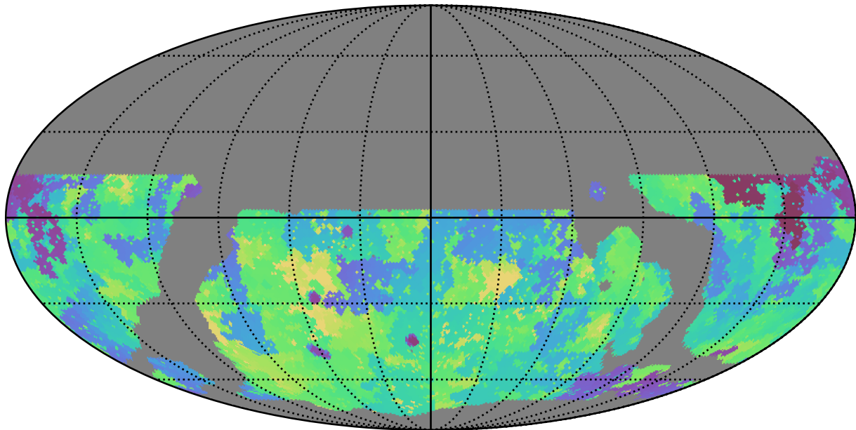
weather_cloudso36v3.4_10yrs WFD g band: Min skyBrightness
