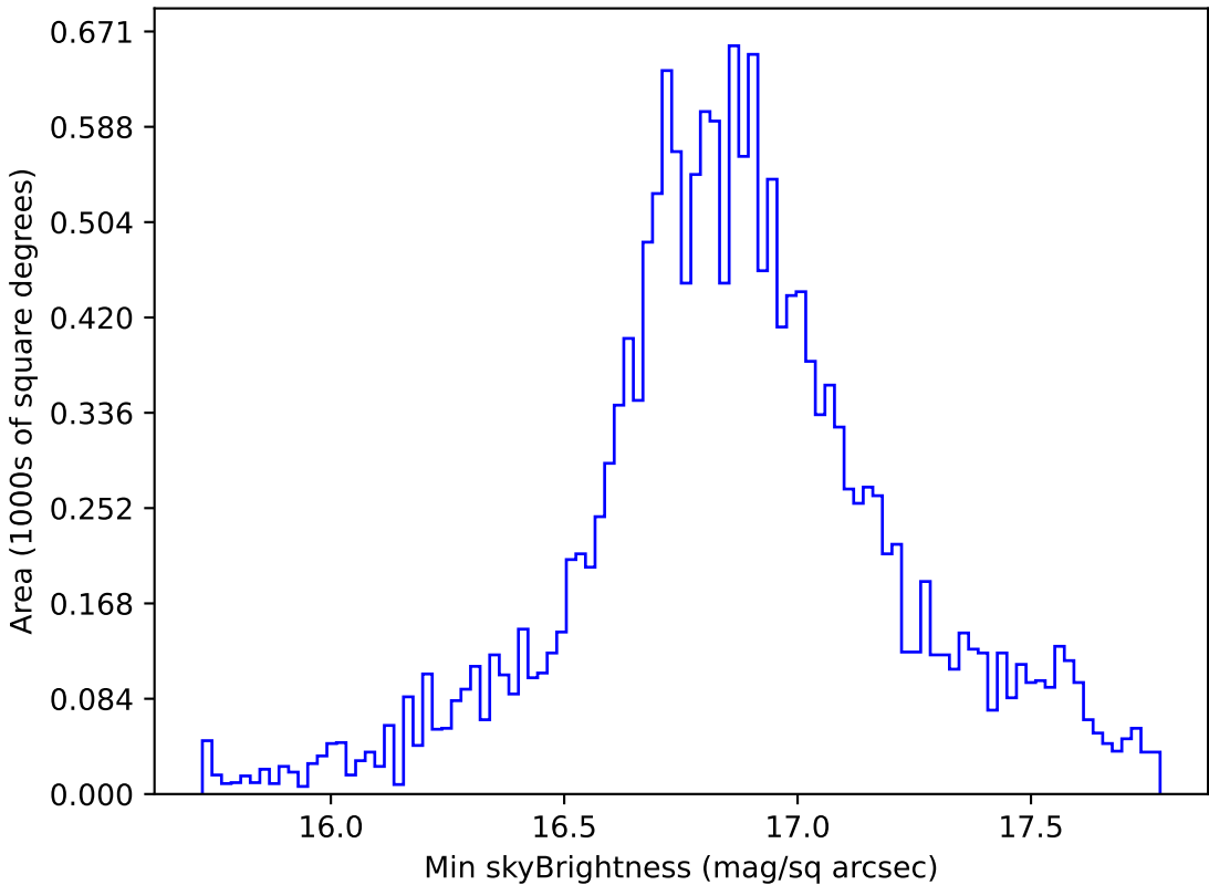
weather_cloudso36v3.4_10yrs WFD all bands: Min skyBrightness
