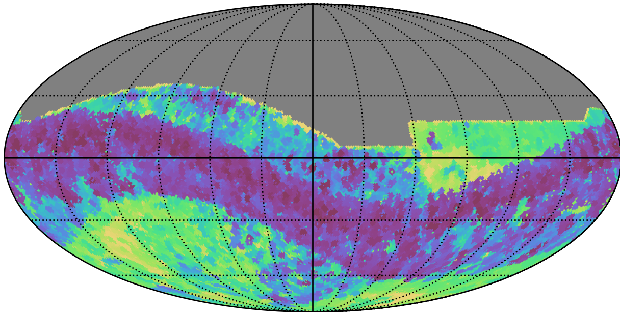
weather_cloudso36v3.4_10yrs All sky z band: Min skyBrightness
