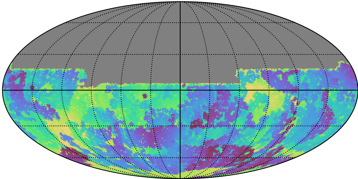
weather_cloudso36v3.4_10yrs All sky u band: Min skyBrightness
