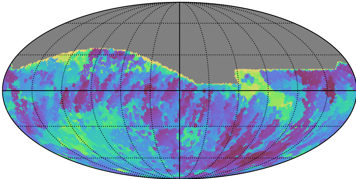
weather_cloudso36v3.4_10yrs All sky r band: Min skyBrightness
