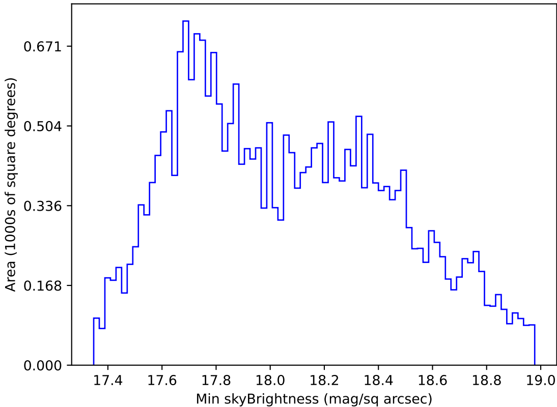
weather_cloudso36v3.4_10yrs All sky i band: Min skyBrightness
