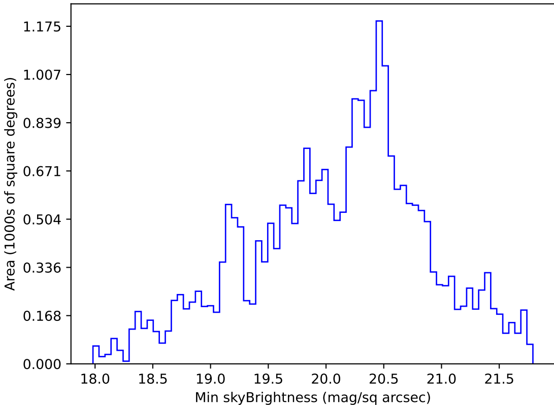
weather_cloudso36v3.4_10yrs All sky g band: Min skyBrightness
