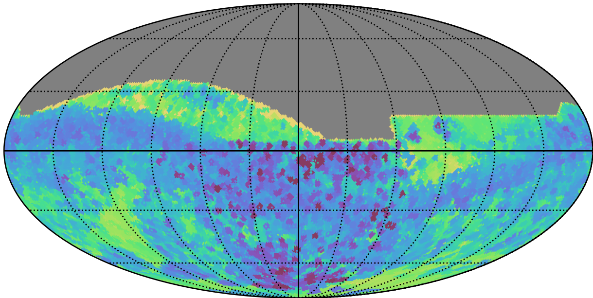
weather_cloudso36v3.4_10yrs All sky all bands: Min skyBrightness
