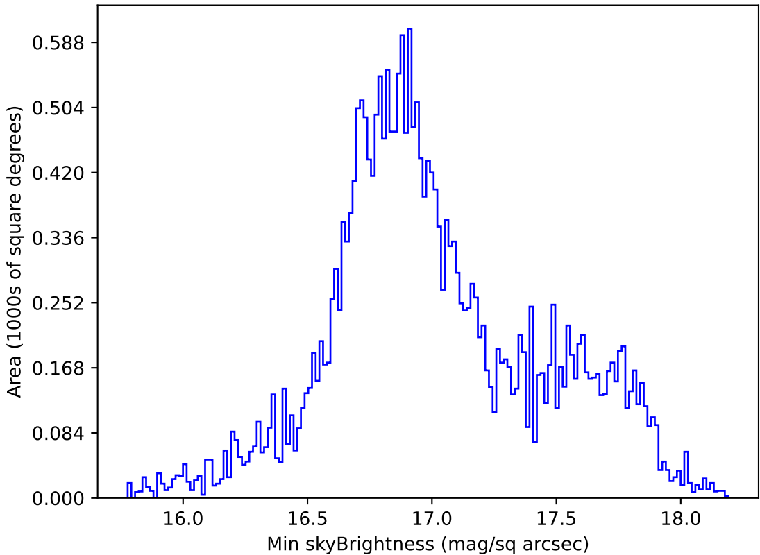
weather_cloudso36v3.4_10yrs All sky all bands: Min skyBrightness
