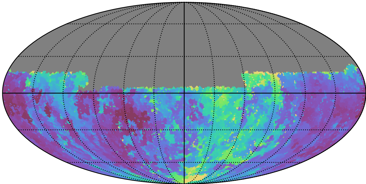
weather_cloudso36v3.4_10yrs Yr 1 u band: Min seeingGeom
