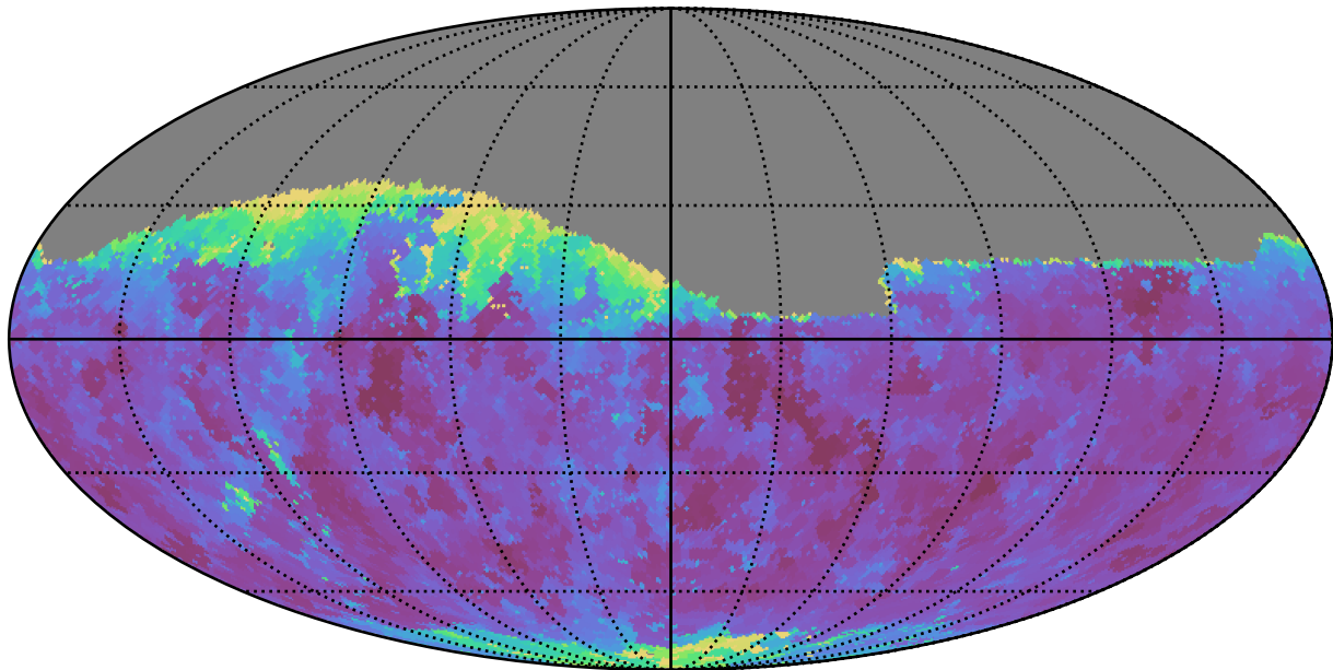
weather_cloudso36v3.4_10yrs Yr 1 r band: Min seeingGeom
