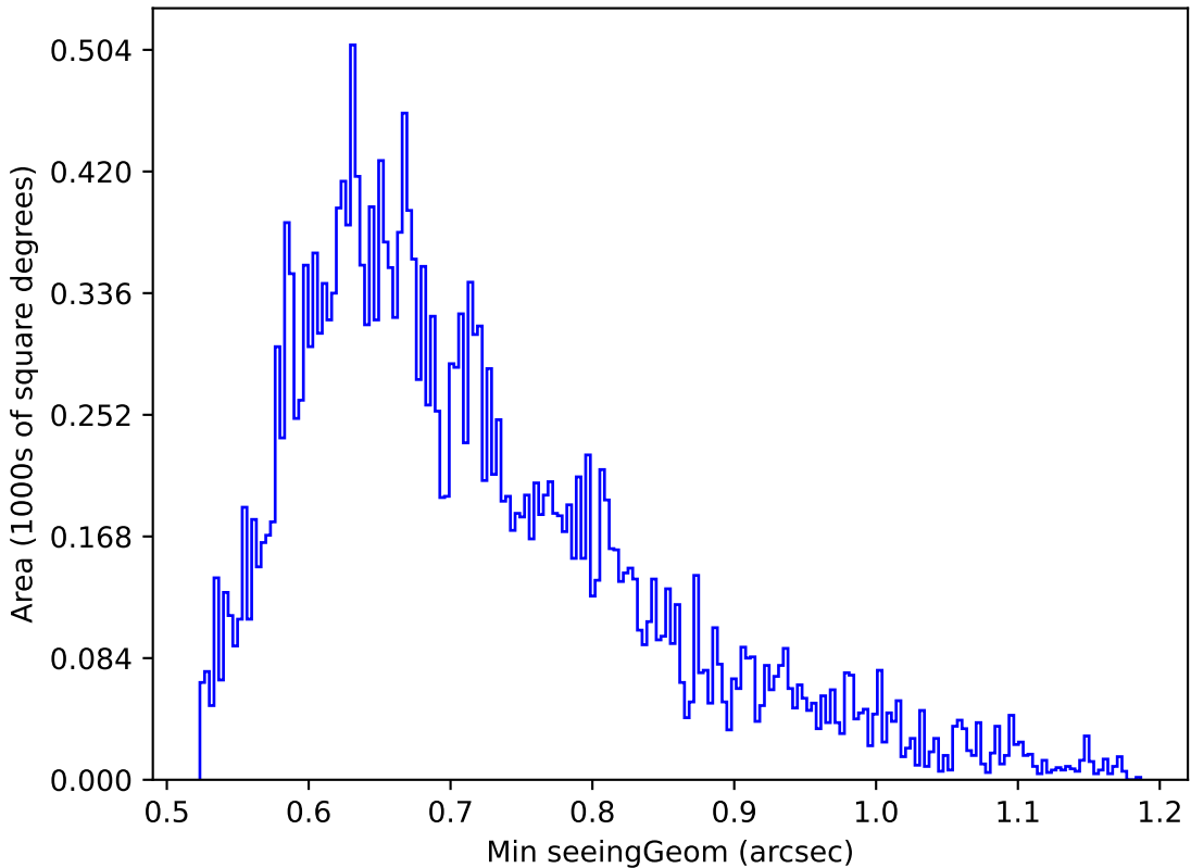
weather_cloudso36v3.4_10yrs Yr 1 g band: Min seeingGeom
