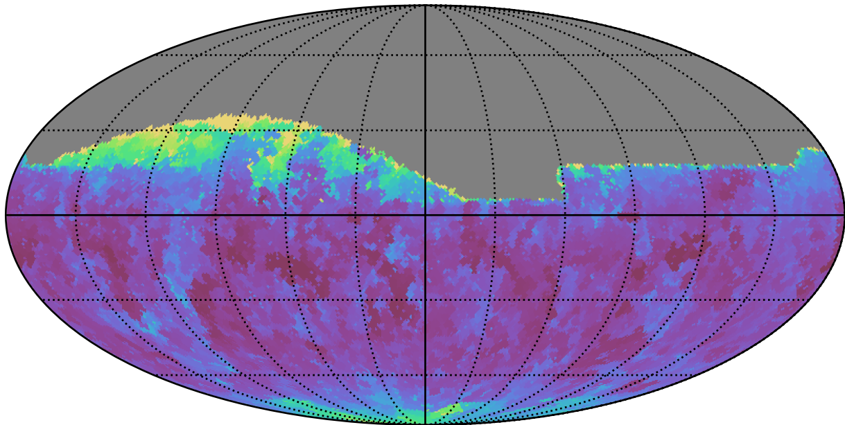
weather_cloudso36v3.4_10yrs Yr 1 all bands: Min seeingGeom
