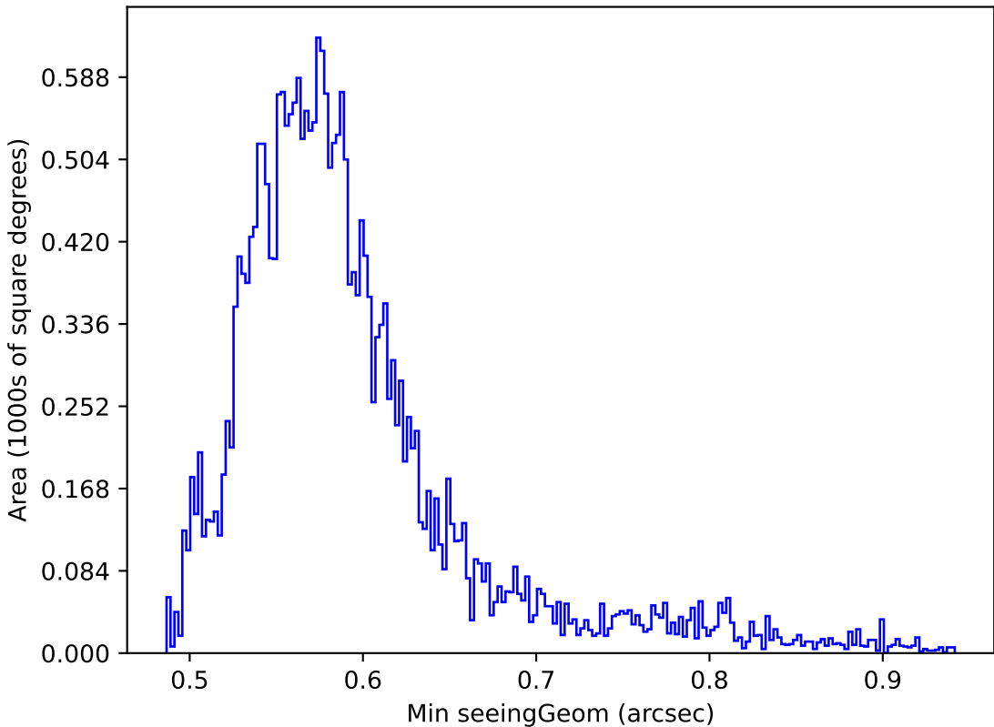
weather_cloudso36v3.4_10yrs Yr 1 all bands: Min seeingGeom
