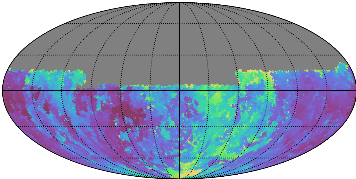
weather_cloudso36v3.4_10yrs Yr 1 u band: Min seeingEff
