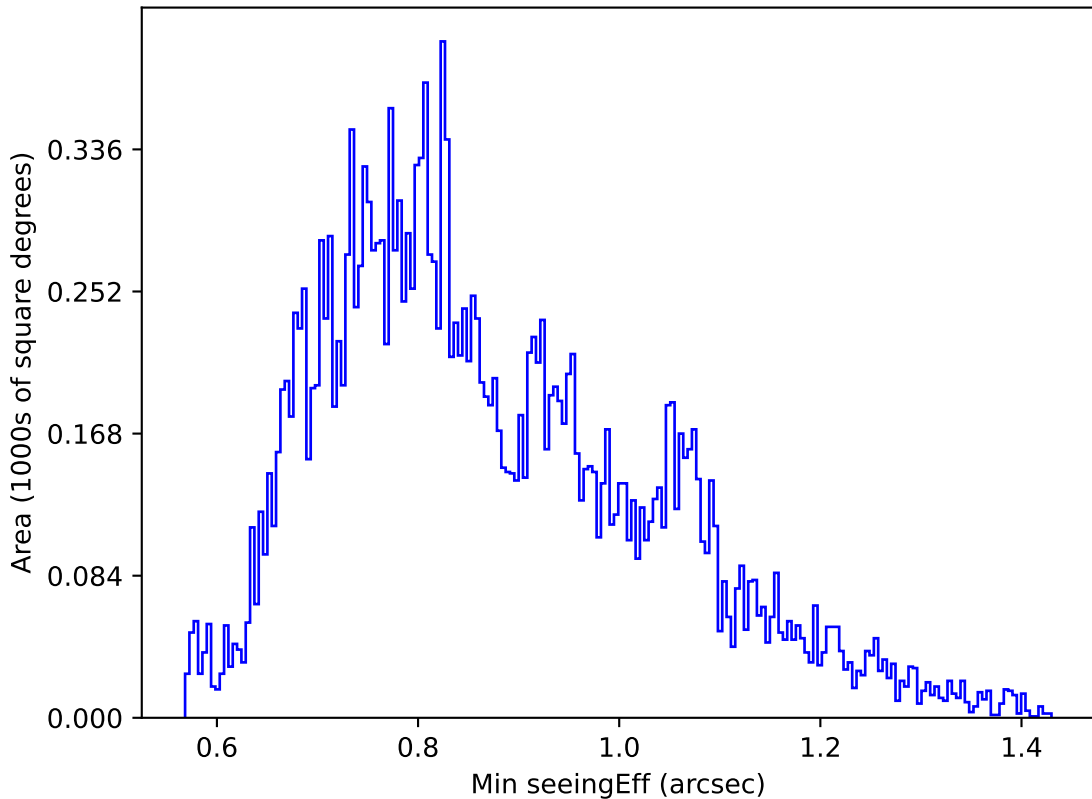
weather_cloudso36v3.4_10yrs Yr 1 u band: Min seeingEff
