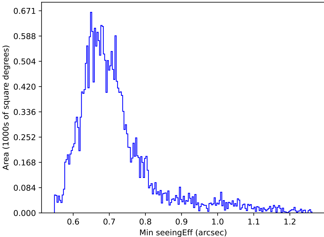
weather_cloudso36v3.4_10yrs Yr 1 i band: Min seeingEff
