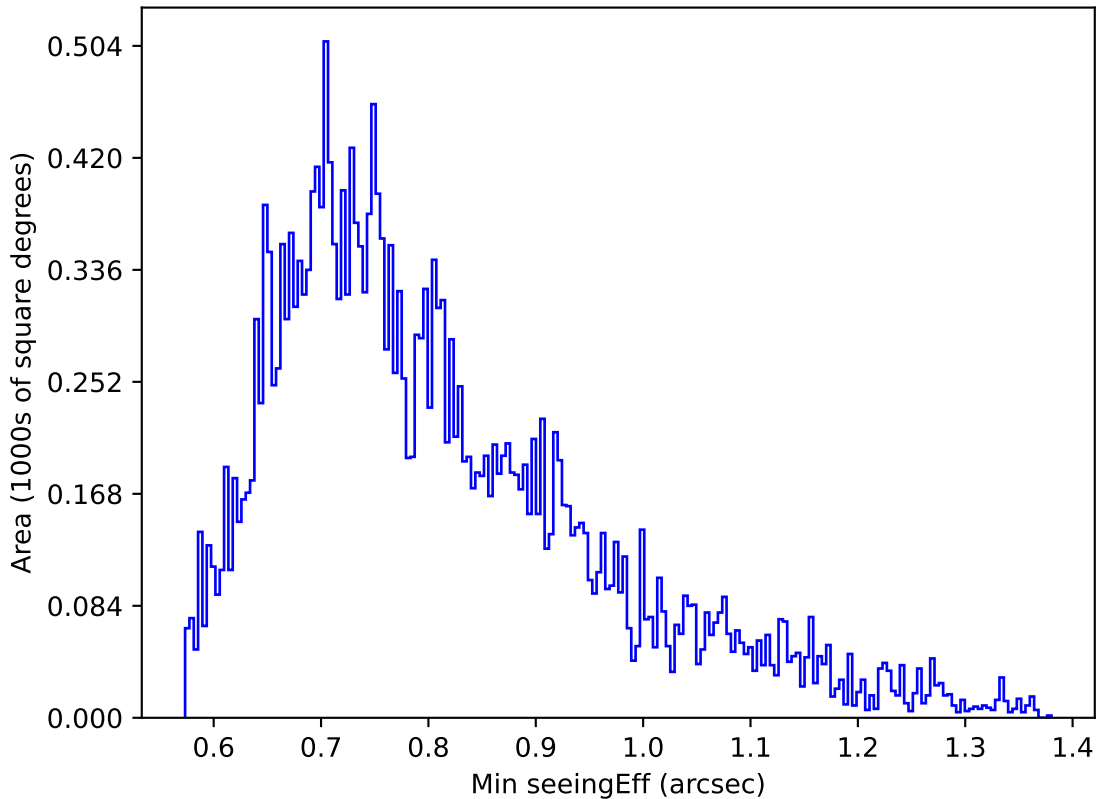
weather_cloudso36v3.4_10yrs Yr 1 g band: Min seeingEff
