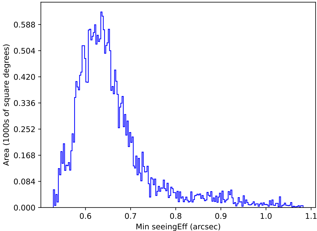
weather_cloudso36v3.4_10yrs Yr 1 all bands: Min seeingEff
