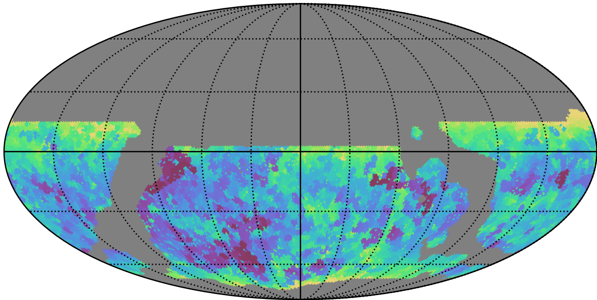
weather_cloudso36v3.4_10yrs WFD z band: Min seeingEff
