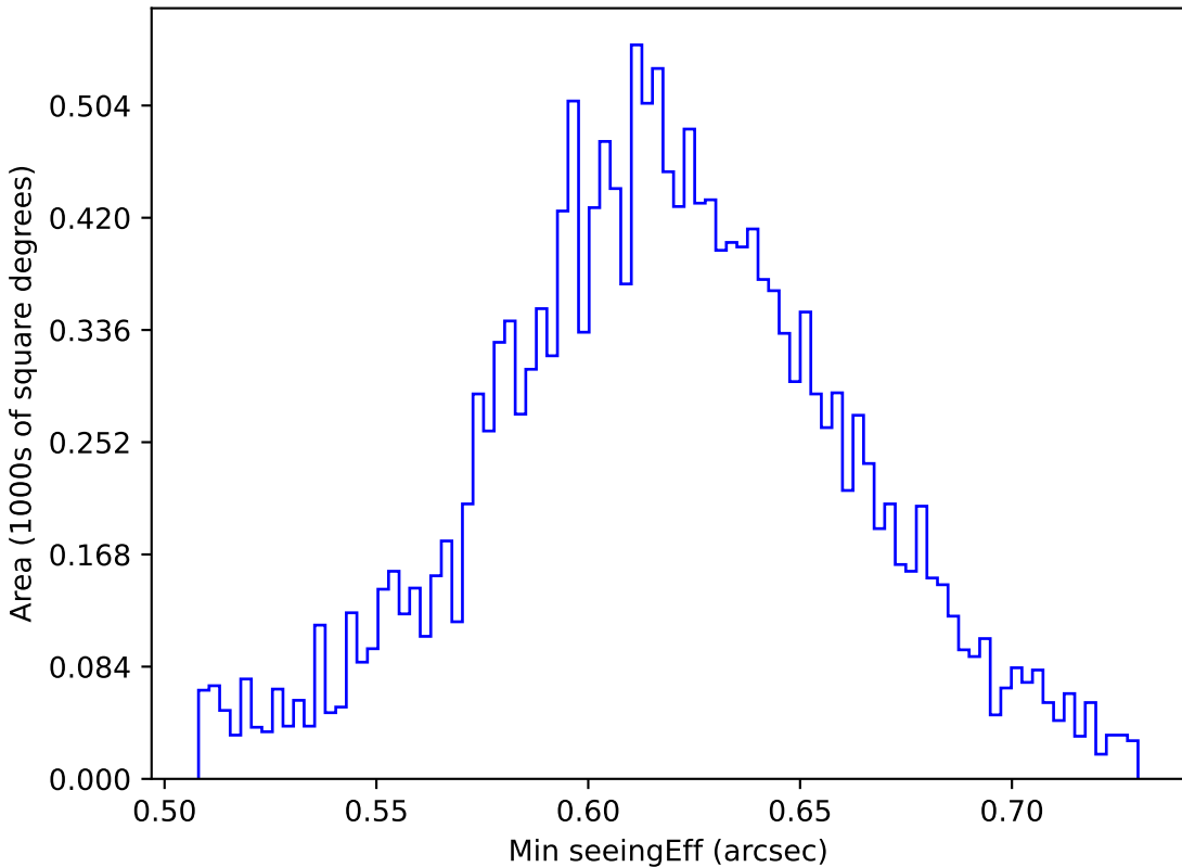
weather_cloudso36v3.4_10yrs WFD z band: Min seeingEff
