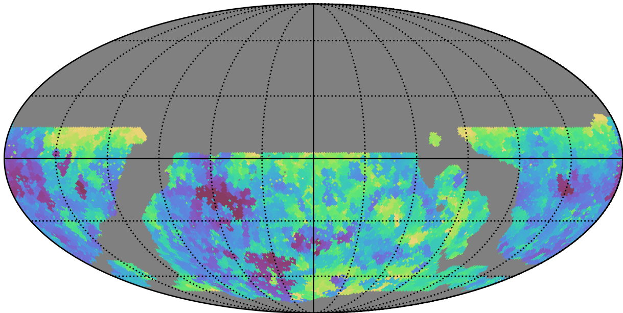
weather_cloudso36v3.4_10yrs WFD u band: Min seeingEff
